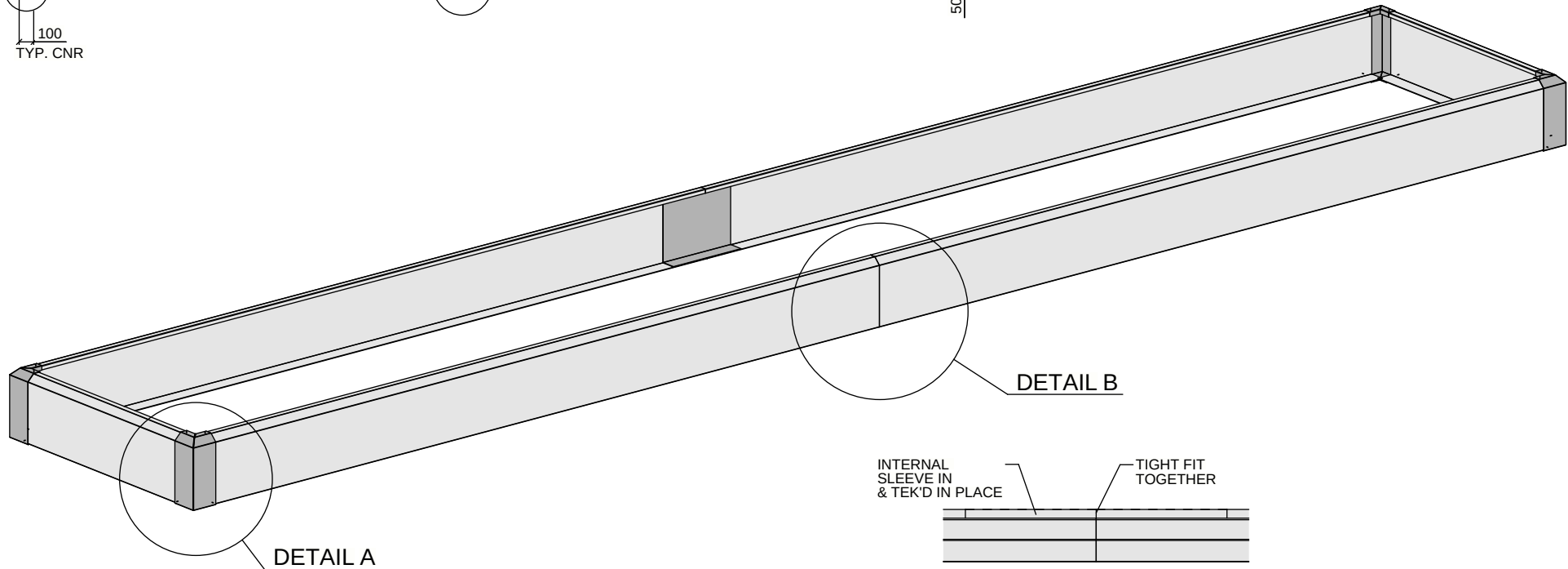
DETAIL-B TYP. JOINER DETAIL
