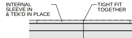
DETAIL-B TYP. JOINER DETAIL
