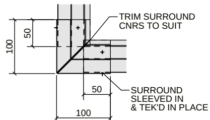
DETAIL-A TYP. CNR DETAIL
